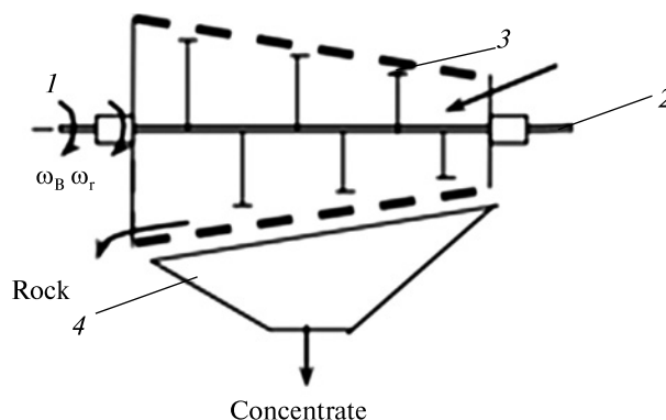
Figure 7. Integrated selective crushing system for separating ice from regolith (1 – conical screen, 2 – shaft, 3 – hammers, 4 – concentrate collector)
