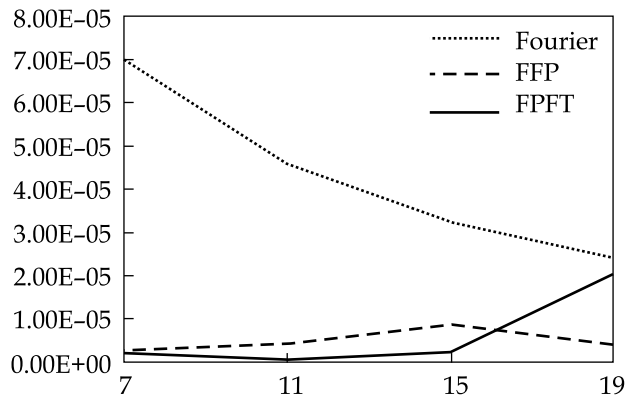
Fig. 6. RMSEa for different types of Fourier polynomials
