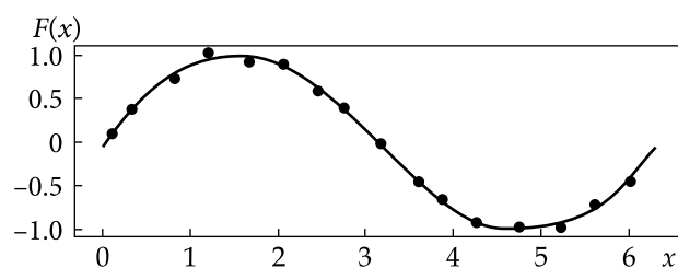
Fig. 2. A Fourier polynomial of degree 10 approximating the sine function represented by 16 points with random noise
