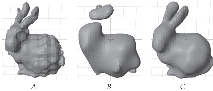
Fig. 7. Visual comparison of Fourier polynomials' modeling quality
