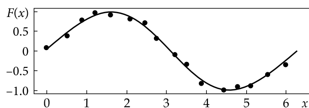
Fig. 1. A Fourier polynomial of degree 5 approximating the sine function represented by 16 points with random noise
