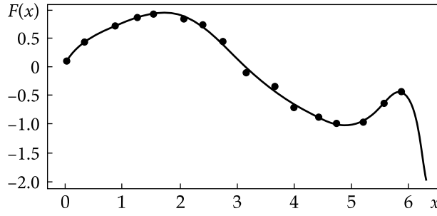
Fig. 4. An FFP of degree 15 approximating the sine function represented by 16 points with random noise
