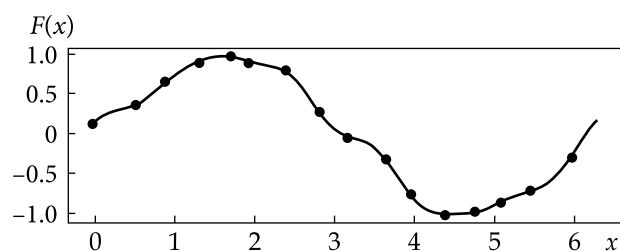
Fig. 3. A Fourier polynomial of degree 15 approximating the sine function represented by 16 points with random noise
